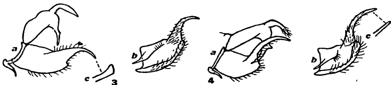
FIG. 3. Borkhausenia enodis n. sp. (a) Lateral view of male genitalia. (b) Inner view of harpe. (c) Apex of harpe from beneath.
