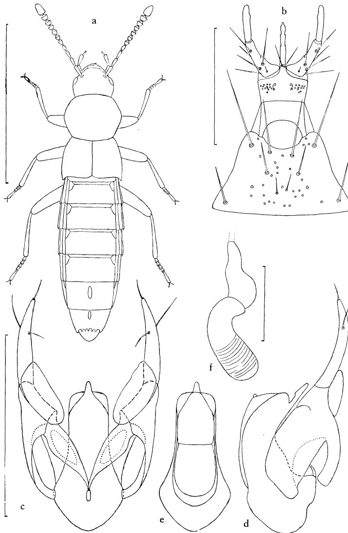
Fig. 20. Halmaeusa antarctica (Kiesenwetter). a, whole insect, scale=2 mm; b, labium, scale=0.2 mm; c, aedeagus, ventral view, scale=0.5 mm; d, aedeagus, lateral view, same scale as c; e, aedeagus, median lobe, dorsal view, same scale as c; f, spermatheca, scale=0.1 mm.
