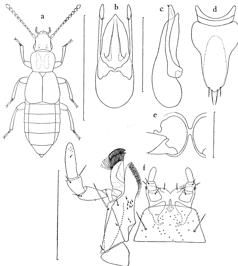
Fig. 7. Arpediomimus kronei (Kiesenwerter). a, whole insect, scale=5 mm; b, aedeagus, ventral view, scale=1 mm; c, aedeagus, lateral view, same scale as b; d, last abdominal sternite of ♂, scale=0.5 mm; e, intermediate coxae, meso- and metasternal processes of ♂, scale=0.5 mm; f, maxilla and labium, scale=0.5 mm.
